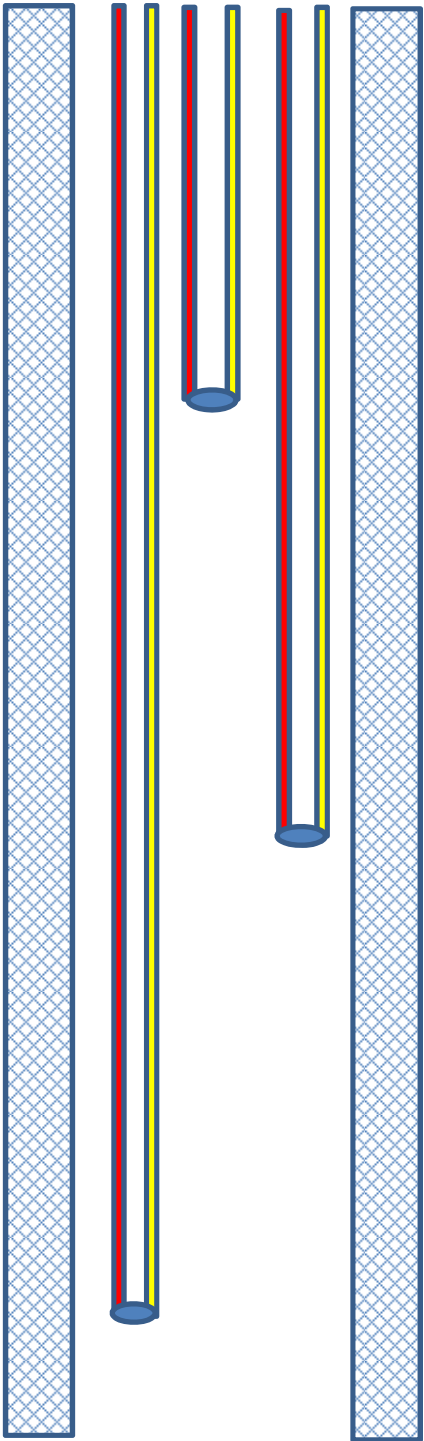
CROSS SECTION OF THE C317 DESIGN MULTIPOINT
